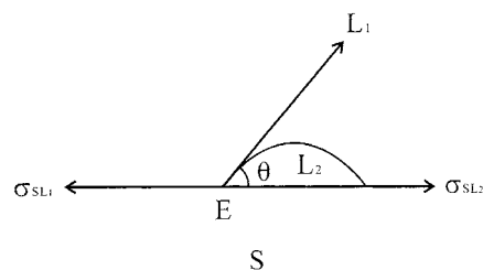
Fig. 2. Schematic representation of three phase contact between the solid S, liquid L_1 and liquid L_2 .
