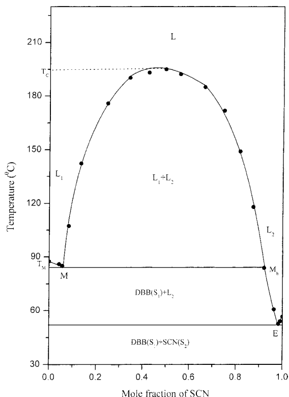
Fig. 1. Phase diagram of p -DBB–SCN system: (●) melting/miscibility temperature.
