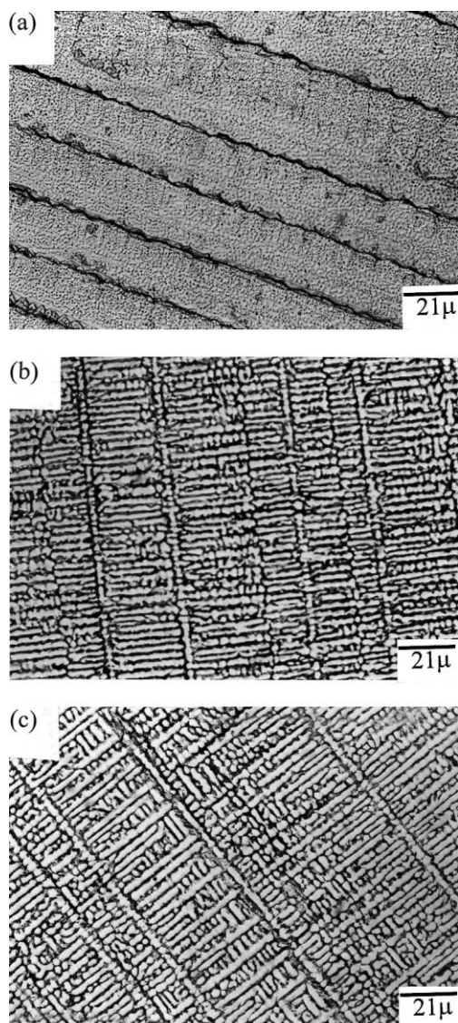
Fig. 3. Optical microphotograph of directionally solidify (a) monotectic, (b) and (c) eutectic.
